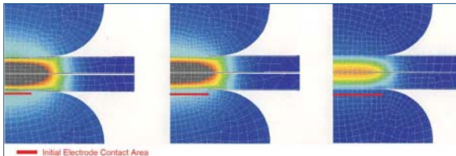
Fig. 3 — A larger weld face reduces current density. Here, the simulations show declining weld nugget size with a constant current and an increasing electrode face diameter (left to right).
