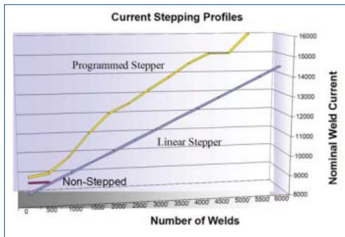
Fig. 5 — Current stepping gradually increases the weld current to compensate for tip wear, allowing for extended use of electrodes. Typical stepping rates range from 0.5–1.0 A per weld increase.
