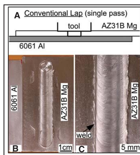
Fig. 7 — Single-pass weld in a conventional lap joint (CL-2) with AZ31 Mg on top of 6061 Al. A — Material position; B — top view overall; C — top view enlarged.
