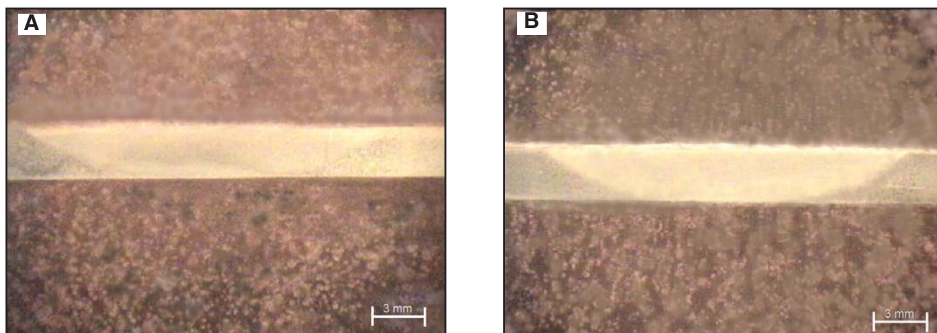
Fig. 1 — Optical macrographs showing the stirred zones (SZ) of the 63/37 brass joints obtained at a rotational speed of 1250 rev/min. Traverse speeds are as follows: A — 100 mm/min; B — 125 mm/min. The plate thickness is 3 mm.
