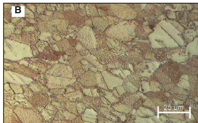
Fig. 3 — Optical micrographs showing the microstructure of 63/37 brass plate used in this study. A — Overall view; B — higher magnification.
