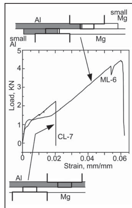
Fig. 16 — Tensile test curves of dual-pass weld CL-7 in conventional lap joint and dual-pass weld ML-6 between AZ31 Mg and 6061 Al in modified lap joint.
