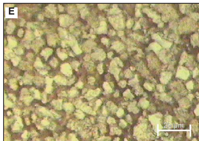
Fig. 5 — Optical micrographs showing the stirred zones (SZ) of the joints obtained with the following weld parameters: A — 1250 rev/min (100 mm/min); B — 1250 rev/min (125 mm/min); C — 1250 rev/min (150 mm/min); D — 1600 rev/min (200 mm/min); and E — 1600 rev/min (225 mm/min.) Note the grain refinement in the SZ.
