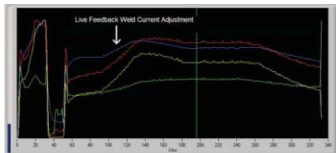
Fig. 6 — During the weld, the weld current (dark blue line) is automatically increased until the resistance signature of the weld indicates that a good weld has been made.
