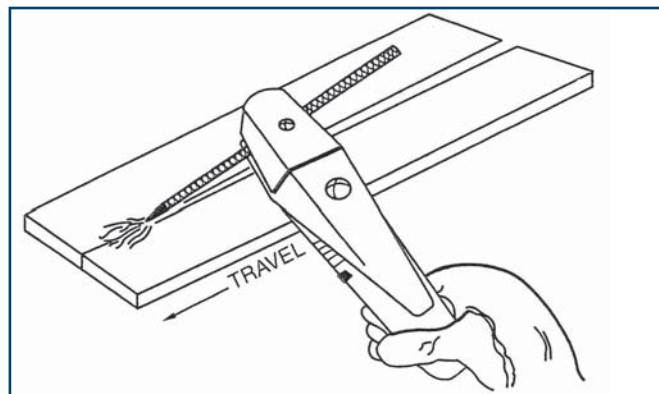
Fig. 1 — Manual air carbon arc gouging in the flat position.
