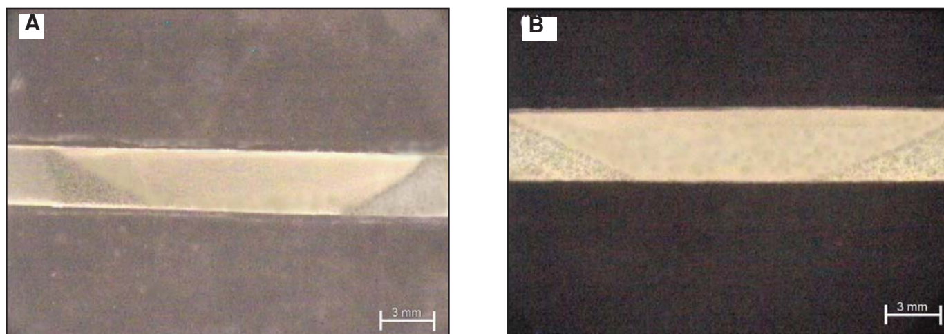
Fig. 2 — Optical macrographs showing the stirred zones (SZ) of the 63/37 brass joints obtained at a rotational speed of 1600 rev/min. Traverse speeds are as follows: A — 175 mm/min; B — 200 mm/min. The plate thickness is 3 mm.
