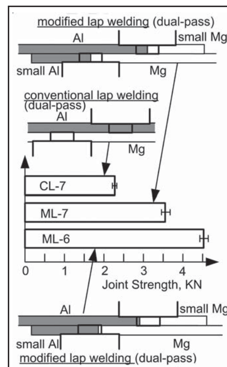
Fig. 15 — Effect of material position on strength of dual-pass welds in lap joint between AZ31 Mg and 6061 Al.
