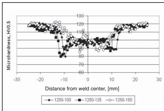
Fig. 6 — Hardness profiles of the joints produced at a rotational speed of 1250 rev/min with different traverse speeds (i.e., 100, 125, and 150 mm/min).
