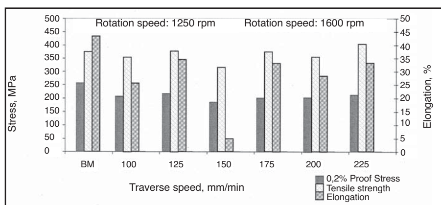
Fig. 10 — Summary of tensile test results.
