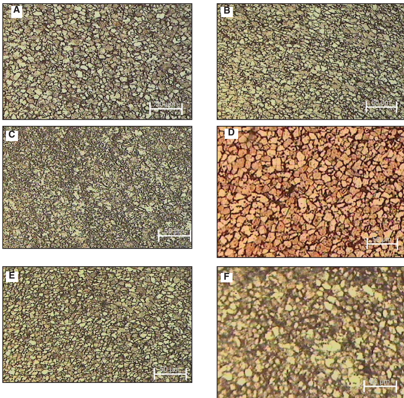
Fig. 4 — Optical micrographs showing the stirred zones (SZ) of the joints obtained with the following weld parameters: A — 1250 rev/min (100 mm/min); B — 1250 rev/min (125 mm/min); C — 1250 rev/min (150 mm/min); D — 1600 rev/min (175 mm/min); E — 1600 rev/min (200 mm/min); and F — 1600 rev/min (225 mm/min). Note the grain refinement in the SZ.
