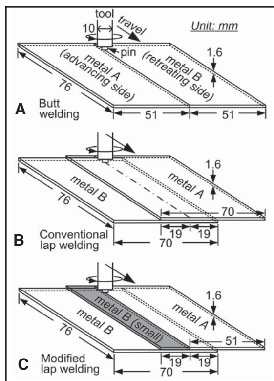
Fig. 1 — Friction stir welding of metal A to metal B. A — Butt joint; B — conventional lap joint; C — modified lap joint (butt joint welding a small piece of metal B to metal A with pin penetration into bottom metal B). Advancing side — material pushed forward by tool; retreating side — material pushed backward.
