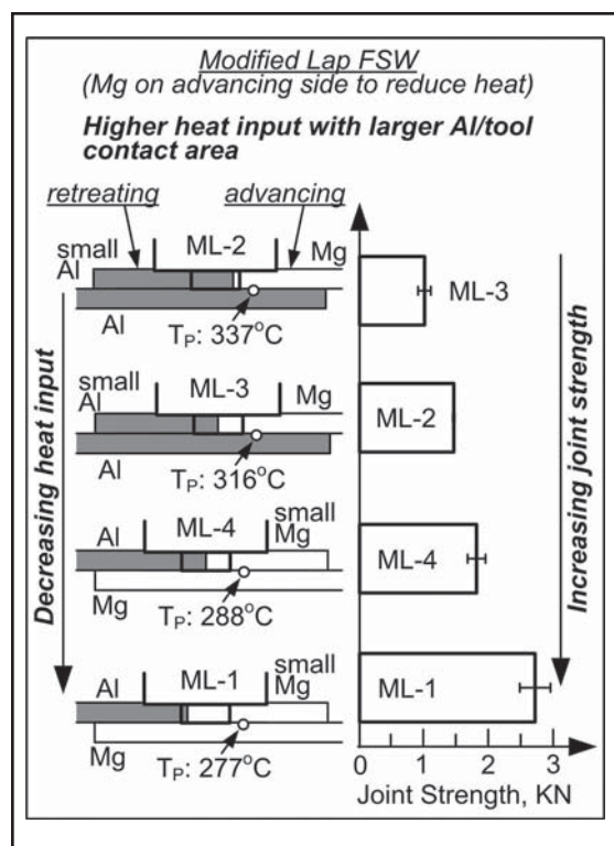
Fig. 12 — Effect of material position on joint strength and heat input in FSW of AZ31 Mg and 6061 Al in a modified lap joint. The thermocouples are 3 mm away from the path of the tool axis and 0.25 mm below the top surface of the lower sheet.
