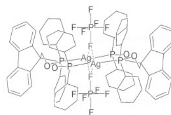
"Noninnocent" \text{PF}_6^- coordination
