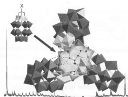
C black, O cyan, WO 4 blue, VO 4 yellow, PO 4 pink
